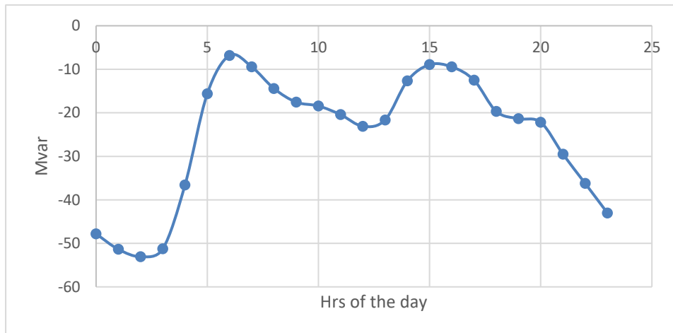
Figure 3-2: Average reactive power generated by HAMILTON STATCOM in each hour of the day from Jan to Dec 2024
