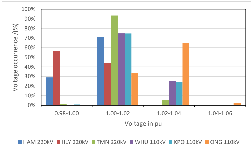
Figure 3-1: Voltage profile of HAM 220kV, HLY 220kV, TMN 220kV, WHU 110kV, KPO 110kV and ONG 110kV from Jan to Dec 2024
