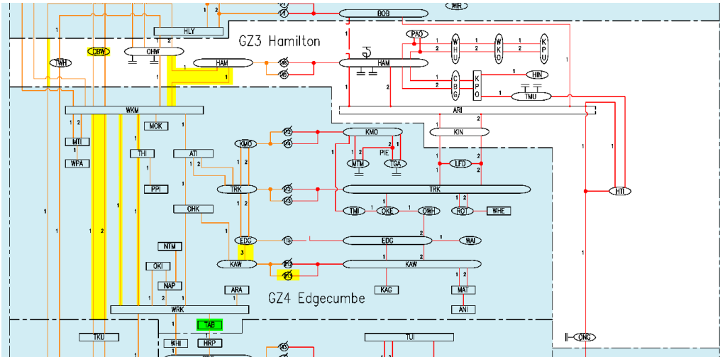
Figure 1-2: Single line diagram of Hamilton Region (Grid Zone 3)
